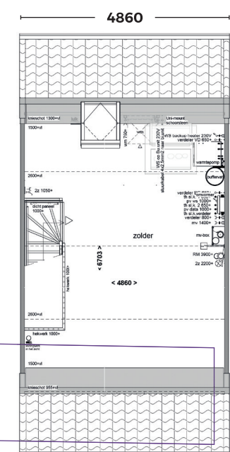
Zolder
